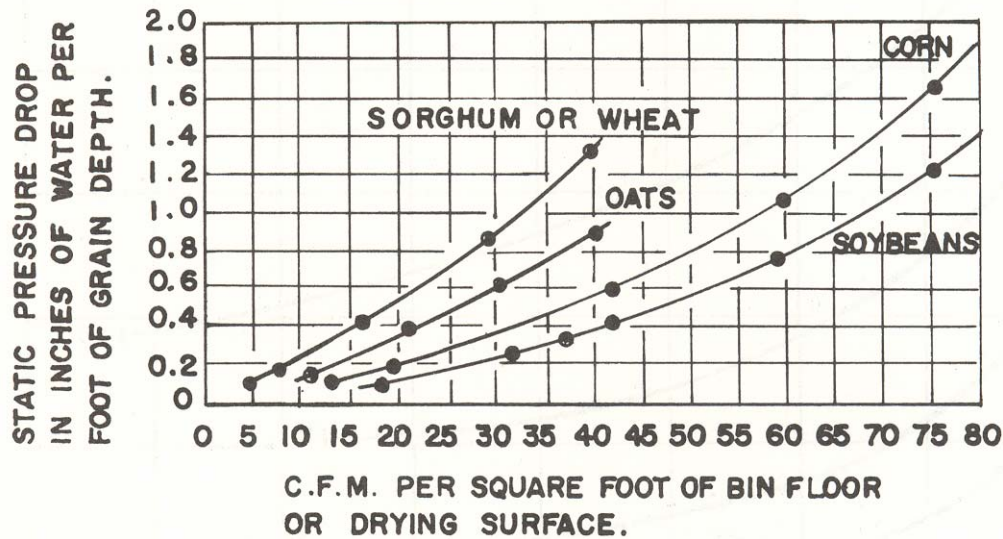
Figure 3. Resistance of grains to air flow, as shown by pressure drop in inches of water per foot of grain (if fines are present in the crop, multiply this data by 1.5).
