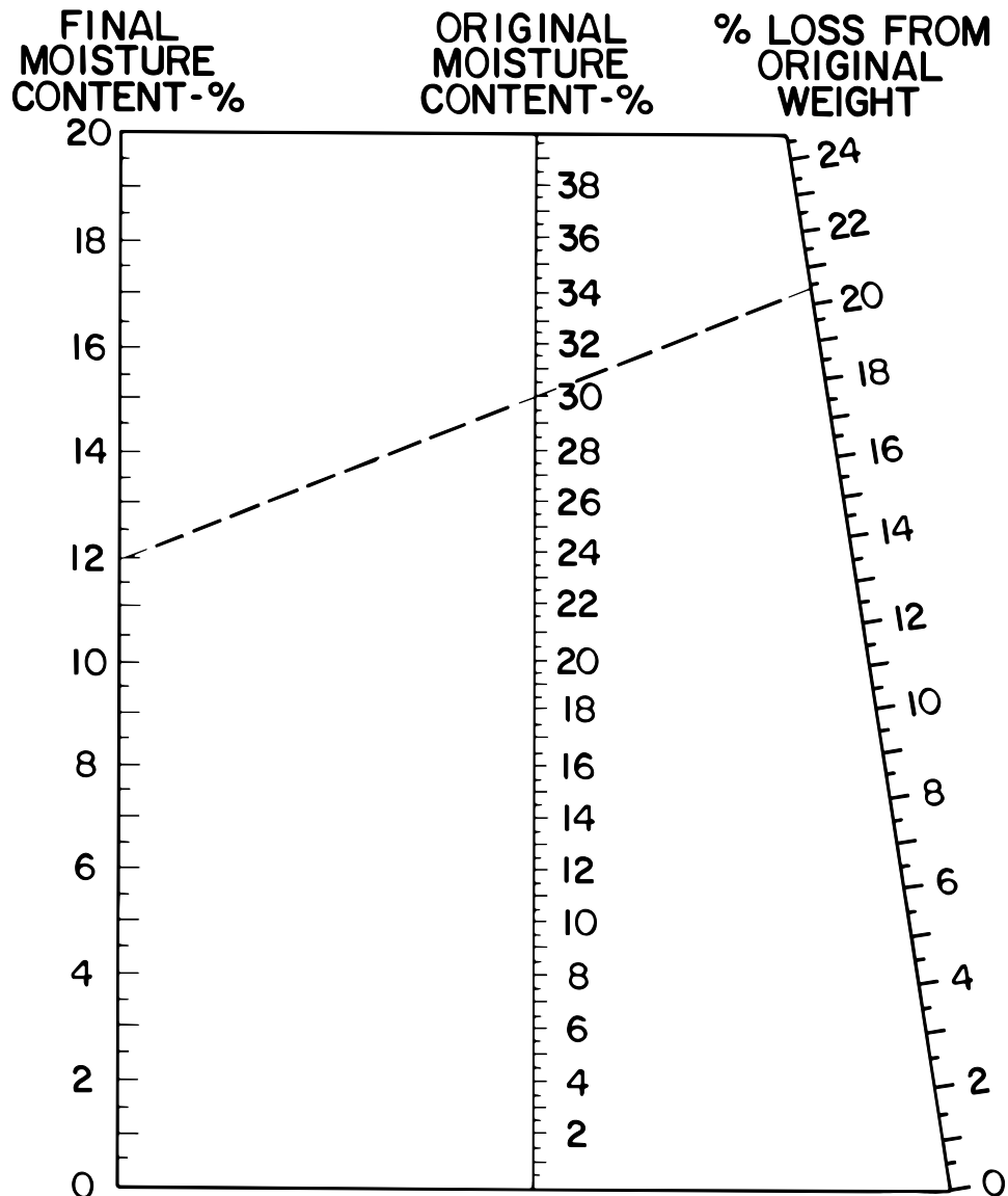
Figure 4. Guide for estimating percent weight lost in grain drying. To use chart, place straight edge at final and original moisture content and read off the percentage loss.
